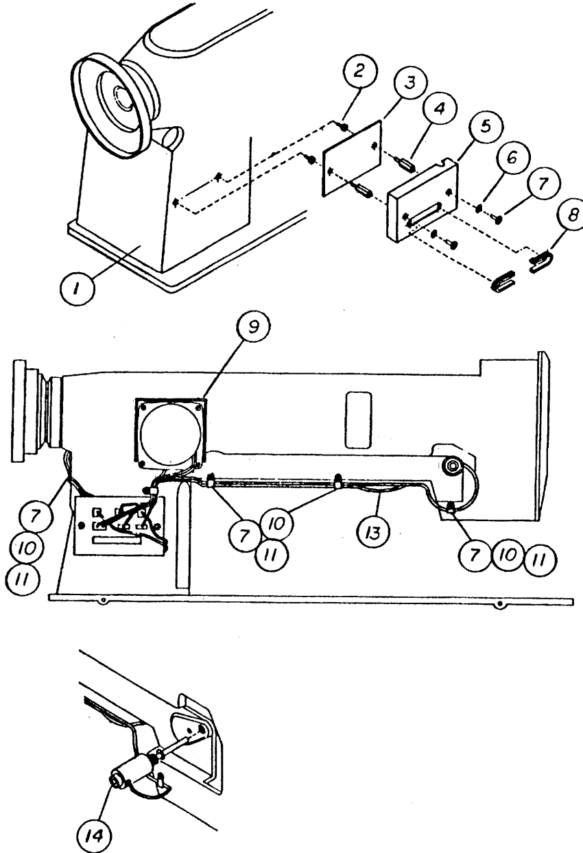
Sewing Head Assembly 1 fig. 12
